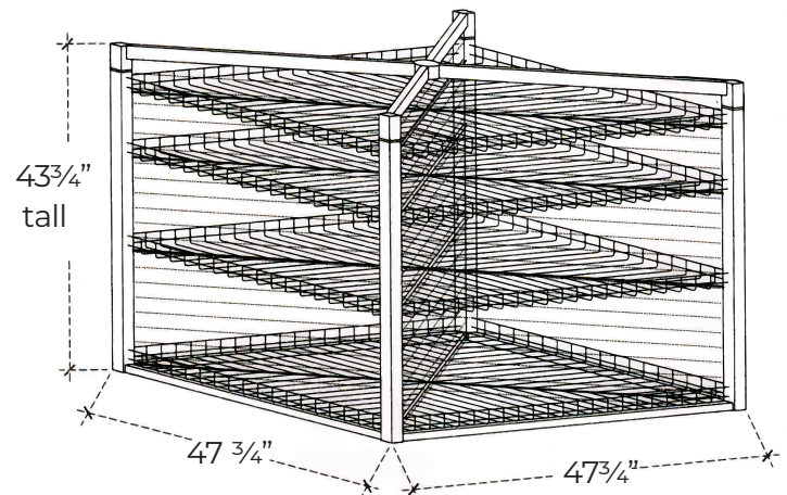
Line Drawing showing dimensions
